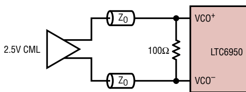
DC-COUPLED 2.5V CML
