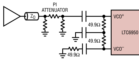
AC-COUPLED RF SINE WAVE OSCILLATOR, OUTPUT >7.5dBm
