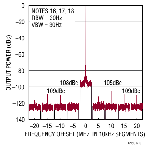
PECLx Spurious Response f_{VCO} = 125MHz , f_{PFD} = 5MHz
