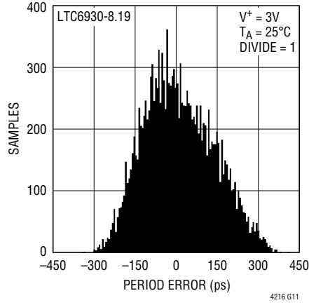
Typical Period Jitter Histogram
