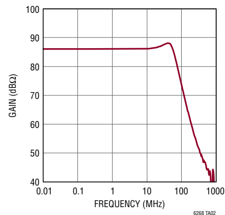
20kΩ TIA Frequency Response
