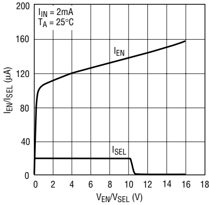
I_{EN} vs V_{EN} and I_{SEL} vs V_{SEL}
