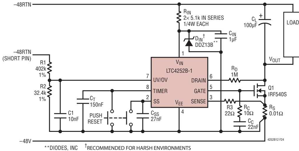
Figure 24. -48V/5A Application
