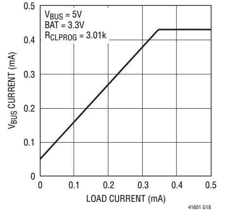
V_{\text{BUS}} Current vs Load Current in Suspend
