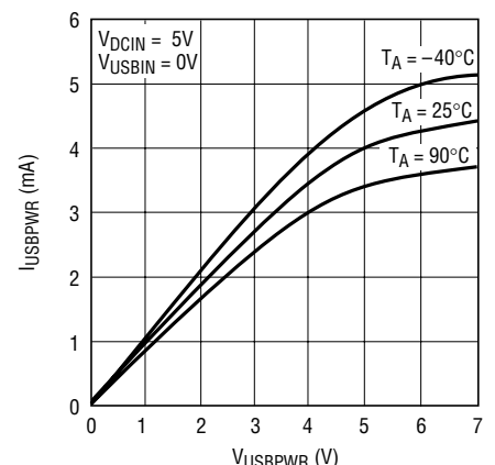
USBPWR Pin I-V Curve
