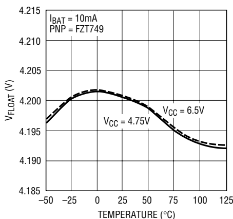
Float Voltage vs Temperature and Supply Voltage
