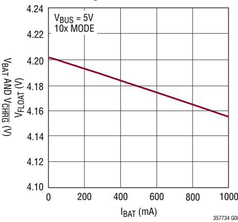
Battery Float Voltage Load Regulation
