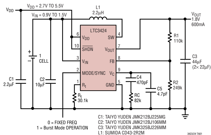
1-Cell to 1.8V at 600mA Step-Up Converter
