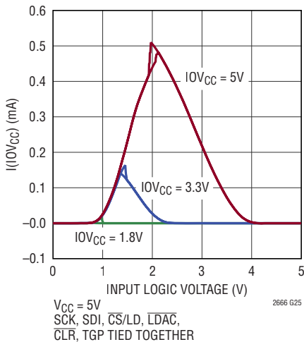
I_{IOV_{CC}} Supply Current vs Logic Voltage
