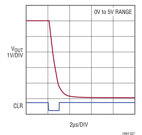
Hardware CLR to Zero-Scale
