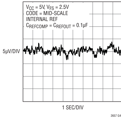
DAC Output 0.1Hz to 10Hz Voltage Noise
