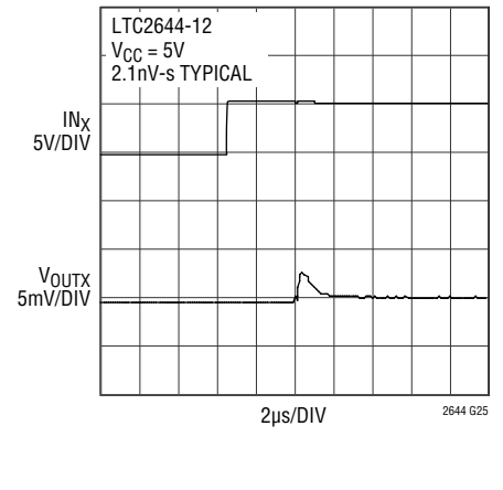
Mid-Scale Glitch Impulse
