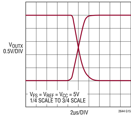
Large-Signal Response
