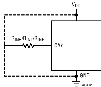
Test Circuit 2
