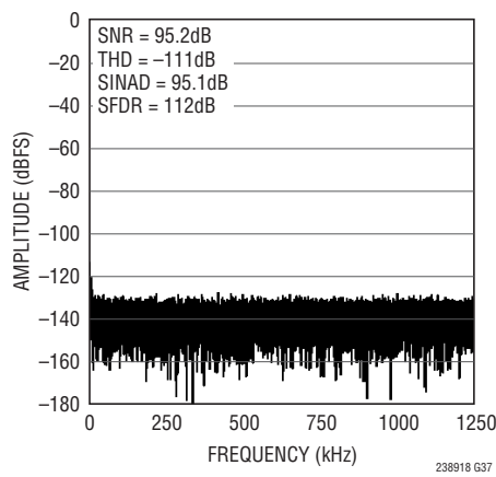
32k Point FFT f_{SMPL} = 2.5\text{Mpsps} , f_{IN} = 2\text{kHz}
