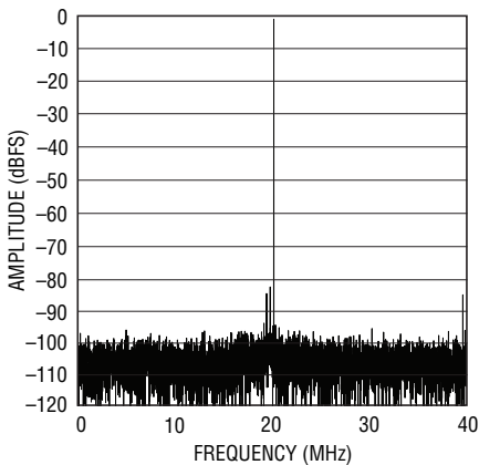
LTC2266-12: 8k Point FFT, f_{IN} = 140\text{MHz} , -1\text{dBFS} , 80Mps
