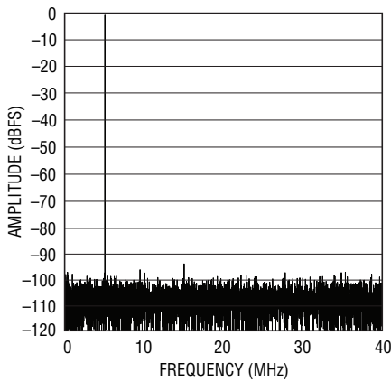
LTC2266-12: 8k Point FFT, f_{IN} = 5\text{MHz} , -1\text{dBFS} , 80Mps
