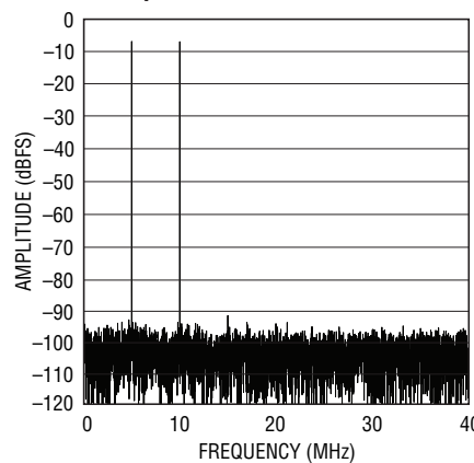
LTC2266-12: 8k Point 2-Tone FFT, f_{IN} = 70\text{MHz}, 75\text{MHz}, -1\text{dBFS}, 80\text{Mps}
