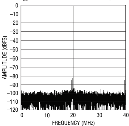
LTC2266-12: 8k Point FFT, f_{IN} = 140\text{MHz}, -1\text{dBFS}, 80\text{Mps}
