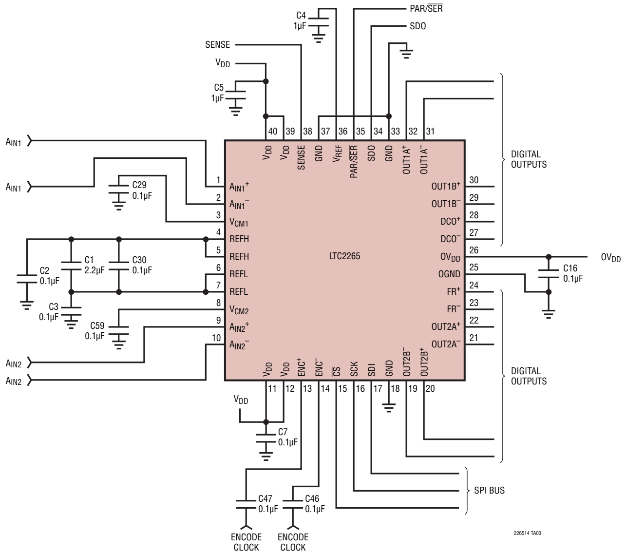
LTC2265 Schematic
