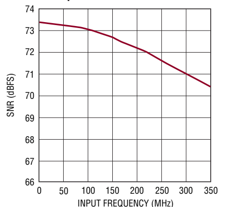
LTC2264-14: SNR vs Input Frequency, -1\text{dBFS} , 2\text{V} Range, 40\text{Mpsps}
