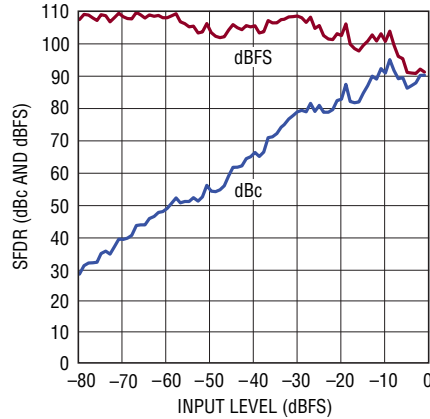
LTC2265-14: SFDR vs Input Level, f_{IN} = 70\text{MHz} , 2V Range, 65Msps
