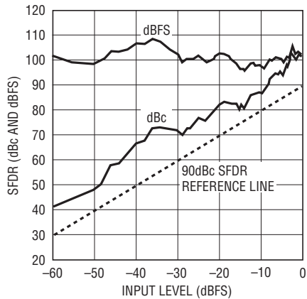
LTC2226: SFDR vs Input Level, f_{IN} = 5\text{MHz} , 2V Range, 25MSPs
