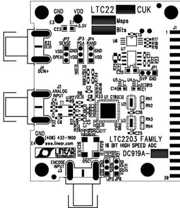
Silkscreen Top
