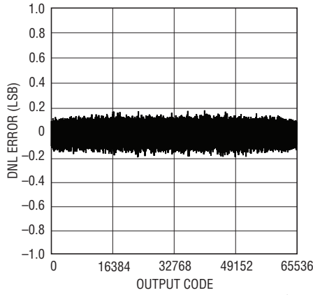
LTC2182: Differential Non-Linearity (DNL)
