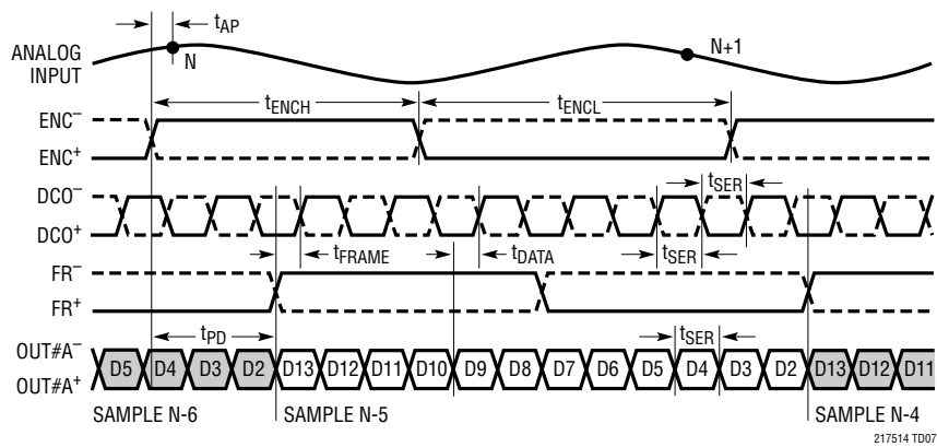
One-Lane Output Mode, 12-Bit Serialization
