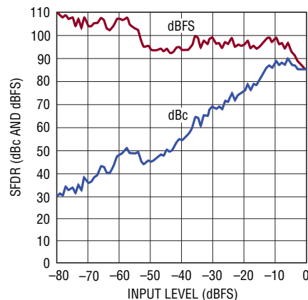
LTC2174-14: SFDR vs Input Level, f_{IN} = 70\text{MHz}, 2\text{V Range}, 105\text{Mps}
