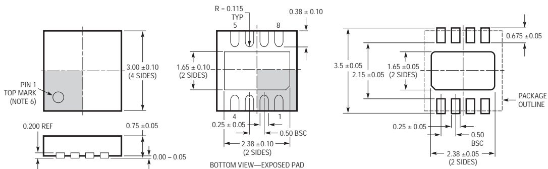
RECOMMENDED SOLDER PAD PITCH AND DIMENSIONS (002) DRN 1203
