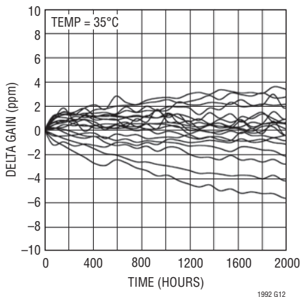
Differential Gain vs Time (Normalized to t = 0 )
