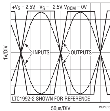
Output Overdrive Recovery (Expanded View)
