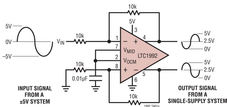
Single-Supply, Single-Ended to Differential Conversion
