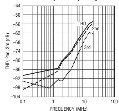
THD, 2nd and 3rd vs Input Frequency
