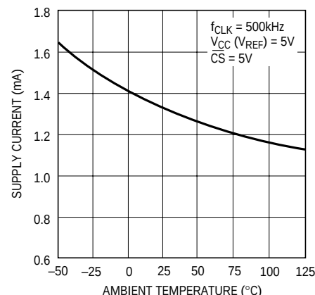
LTC1091 Supply Current vs Temperature
