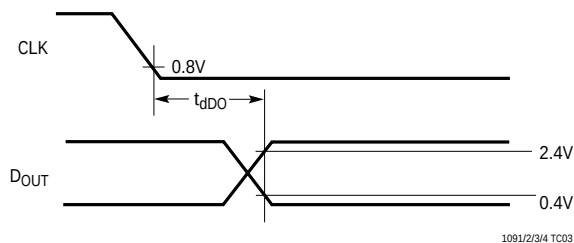
Voltage Waveforms for D_{OUT} Delay Time, t_{dO}
