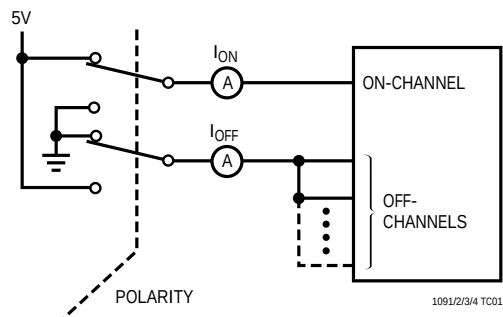
On- and Off-Channel Leakage Current
