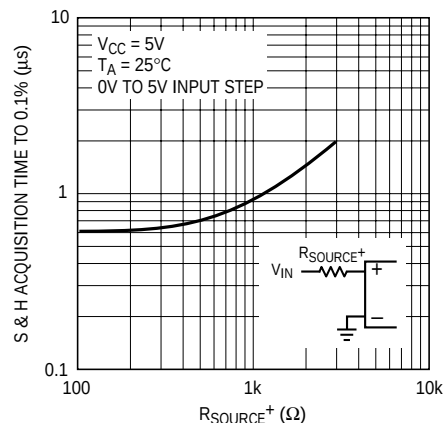
LTC1091/LTC1092/LTC1093/LTC1094 Sample-and-Hold Acquisition Time vs Source Resistance
