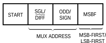
LTC1091 DATA INPUT ( D_{IN} ) WORD:
