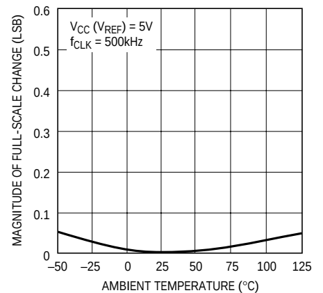
Change in Full-Scale Error vs Temperature
