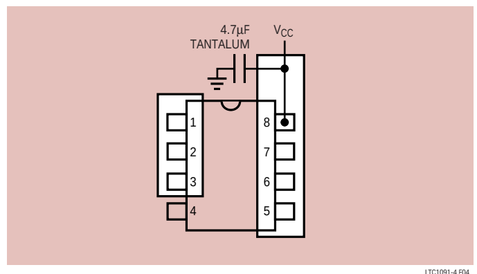
Figure 4. Example Ground Plane for the LTC1091
