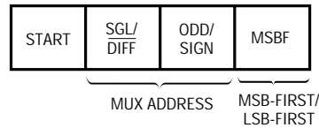
LTC1093/LTC1094 DATA INPUT ( D_{IN} ) WORD:
