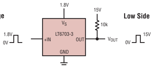
Level Translator Low Voltage to High Voltage
