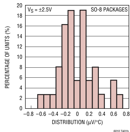
Distribution of Offset Voltage Drift
