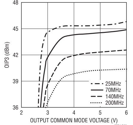
Two-Tone OIP3 vs V_{CCO} , for G_{MAX} -3.875dB
