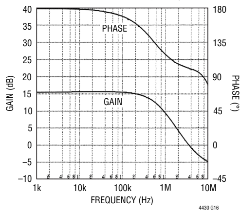
Opto Driver Inverting Closed Loop Gain and Phase vs Frequency
