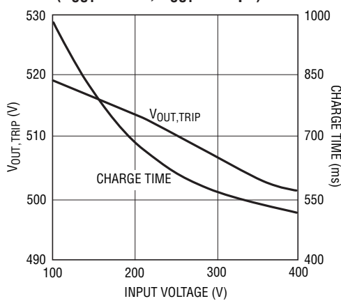
Output Trip Voltage and Charge Time ( V_{OUT} = 500V , C_{OUT} = 220\mu F )
