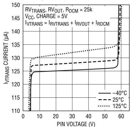
V TRANS Supply Current
