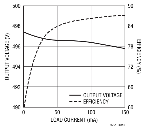
Load Regulation and Efficiency
