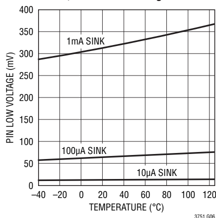
DONE, FAULT Pin Voltage Low
