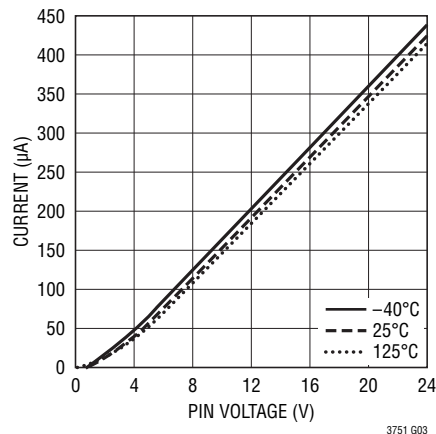
CHARGE Pin Current
