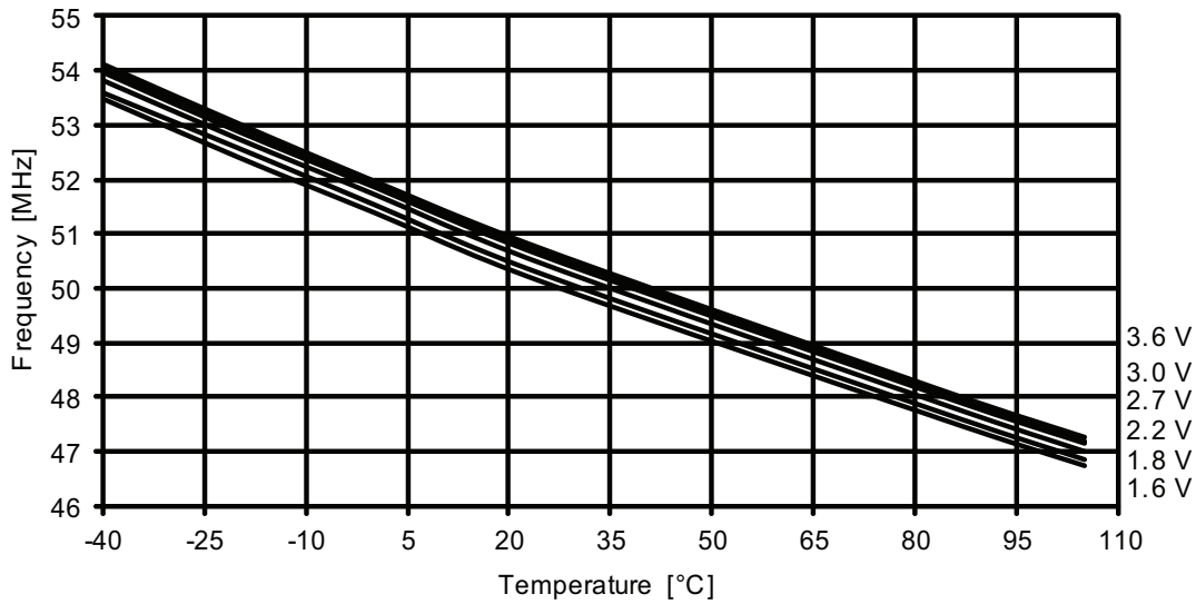
Figure 37-244. 48MHz internal oscillator frequency vs. temperature. DFLL disabled.
