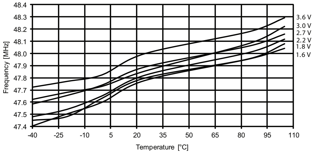
Figure 37-245. 48MHz internal oscillator frequency vs. temperature. DFLL enabled, from the 32.768kHz internal oscillator.
