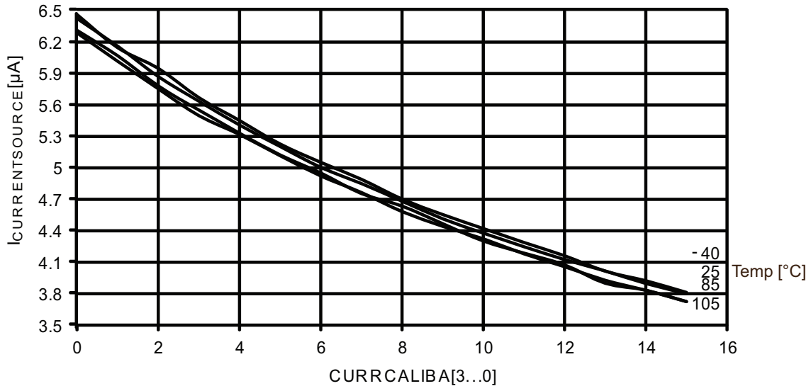
Figure 37-139. Analog comparator current source vs. calibration value.
