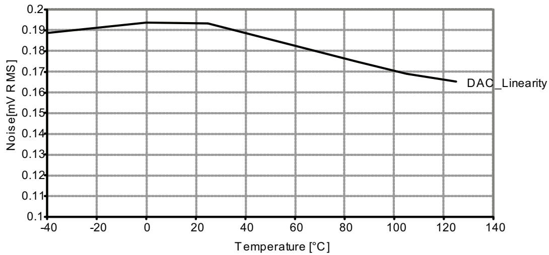
Figure 37-216. DAC noise vs. temperature.
