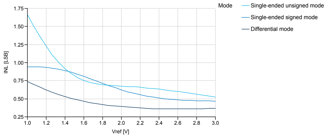
Figure 37-38. ADC INL vs. V_{REF} T = 25^{\circ}\text{C} , V_{CC} = 3.6\text{V} , external reference
