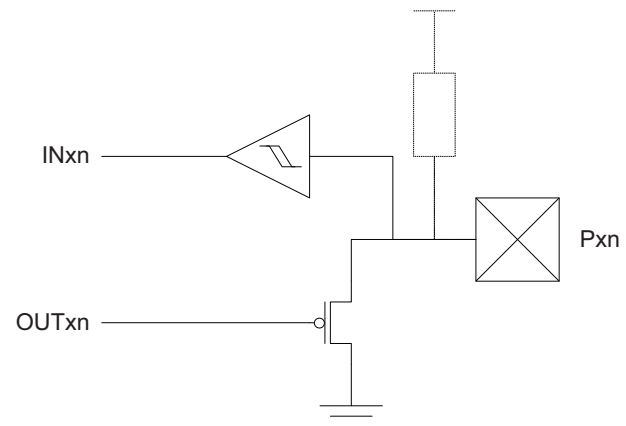
Figure 16-6. I/O Configuration - Wired-AND with Optional Pull-up
