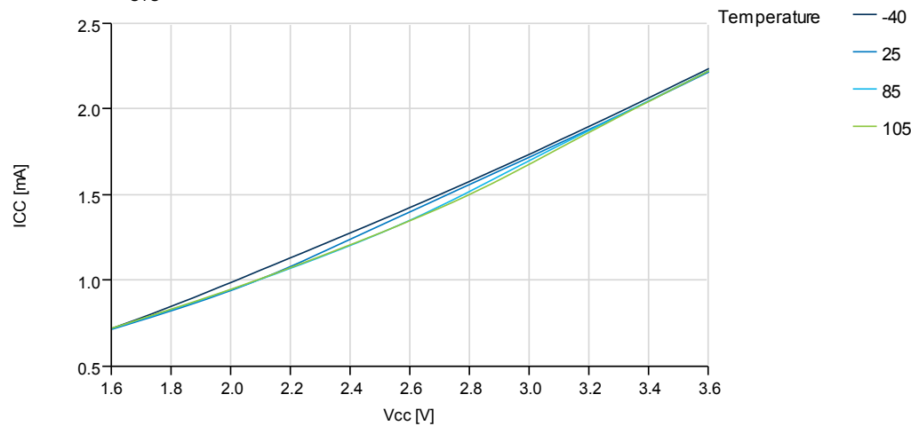
Figure 37-6. Active Mode Supply Current vs. V_{CC} f_{SYS} = 8\text{MHz} internal oscillator
