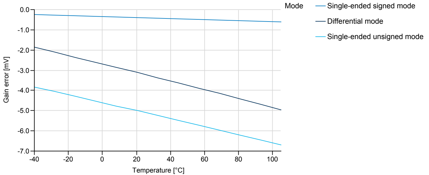
Figure 37-43. ADC Gain Error vs. Temperature
