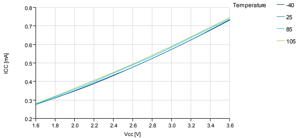
Figure 37-5. Active Mode Supply Current vs. V_{CC} f_{SYS} = 8\text{MHz} internal oscillator prescaled to 2MHz
