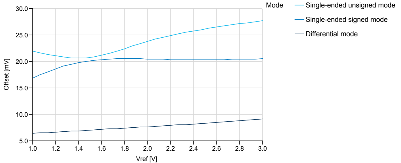
Figure 37-45. ADC Offset Error vs. V_{REF}
