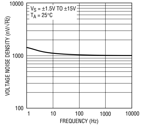
Voltage Noise Density vs Frequency
