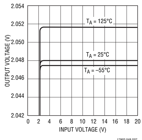
Line Regulation
