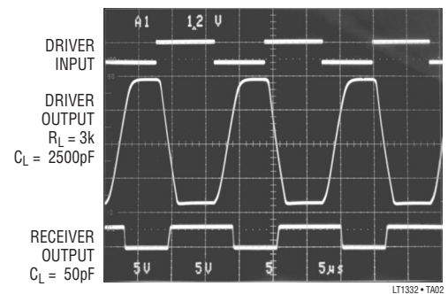
Output Waveforms
