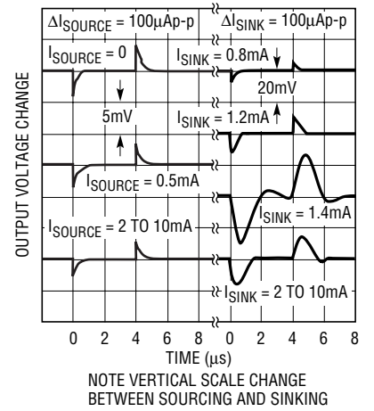
Load Transient Response CLOAD = 1000pF
