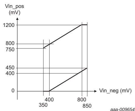
Fig 49. Positive input voltage as a function of the externally supplied negative voltage V_{in\_neg} (on pin ADCHS_NEG)
