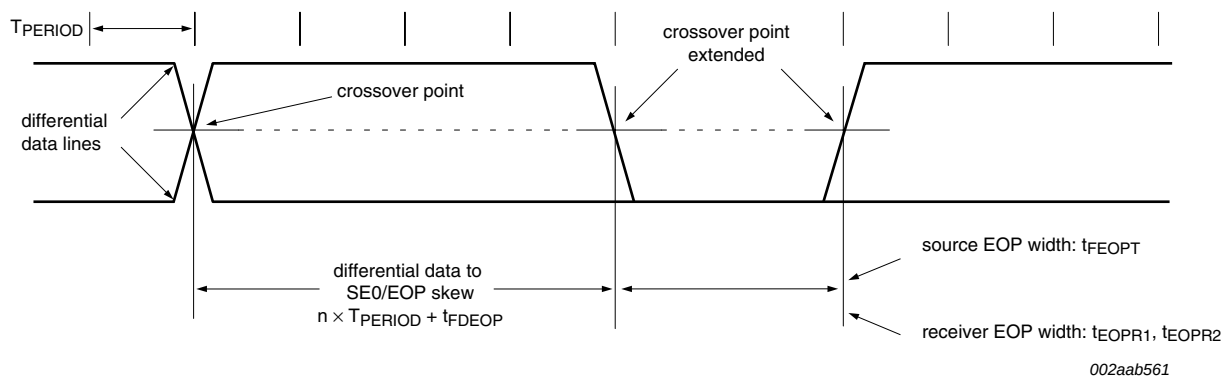
Fig 23. Differential data-to-EOP transition skew and EOP width
