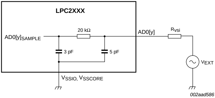
Fig 20. Suggested ADC interface - LPC2470 AD0[y] pin
