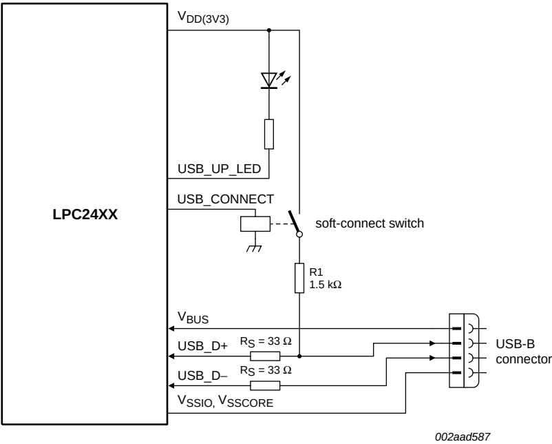
Fig 23. LPC2470 USB interface on a self-powered device
