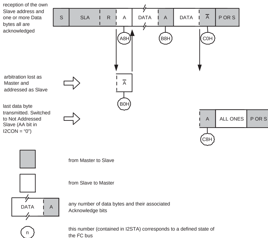
Fig 57. Format and states in the Slave Transmitter mode
