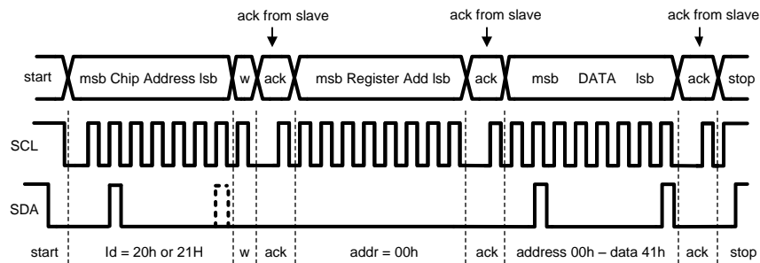
Figure 26. I 2 C Chip Address
