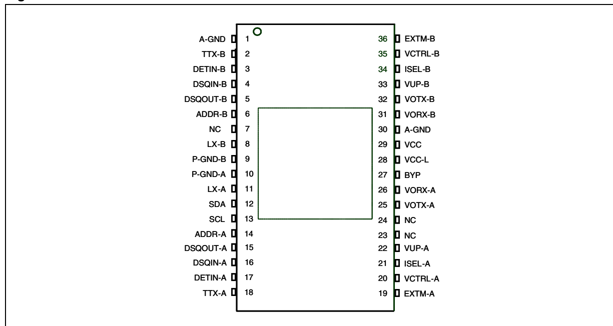
Figure 3. Pin connections
