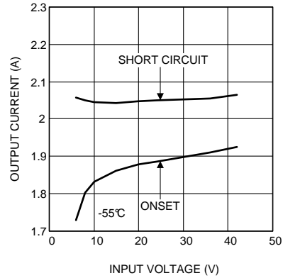
Figure 32. Current Limit 3.3 V OUT at -55°C
