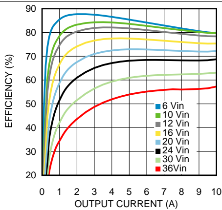
Figure 7. Efficiency 1.8-V Output at 25°C
